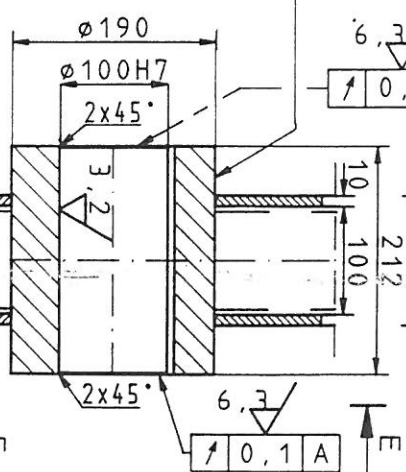
Detail C Skala 1:5
